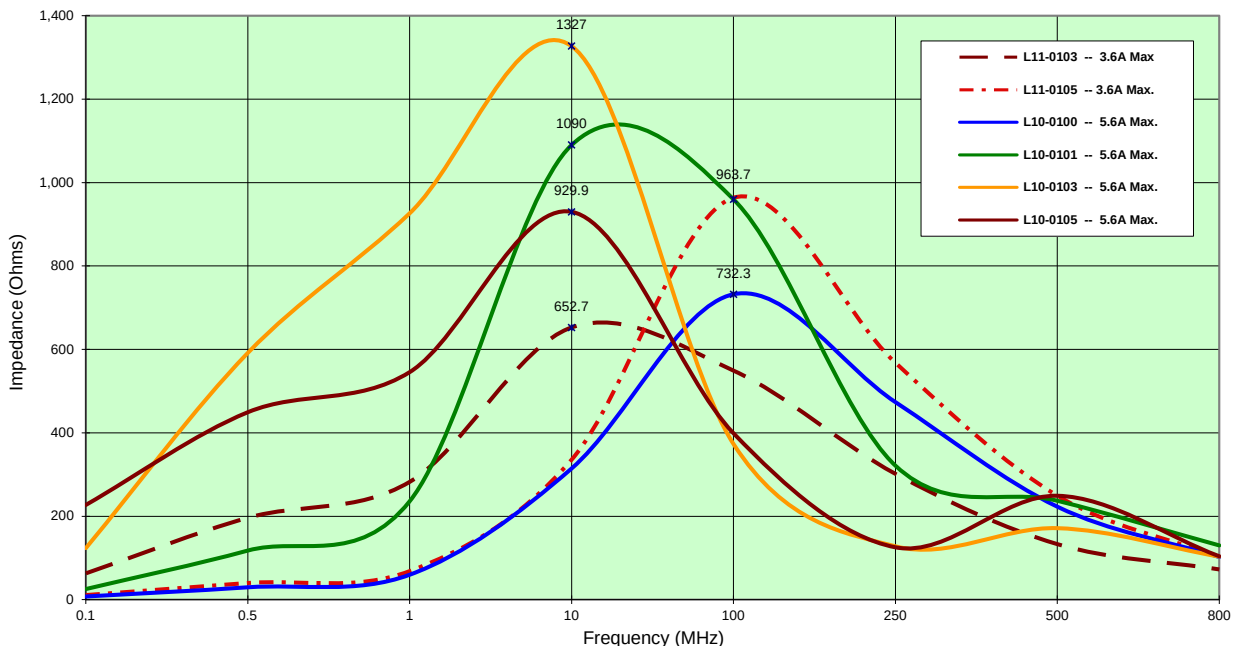
Impedance vs Frequency - BH QTR-Paks (L10-) and 8th-Paks (L11-)
