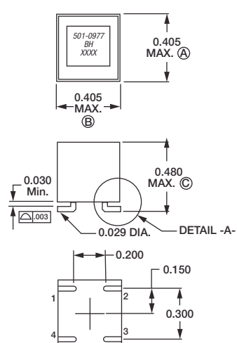
501-0977 MECHANICAL
