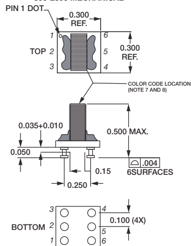
500-2506 MECHANICAL
