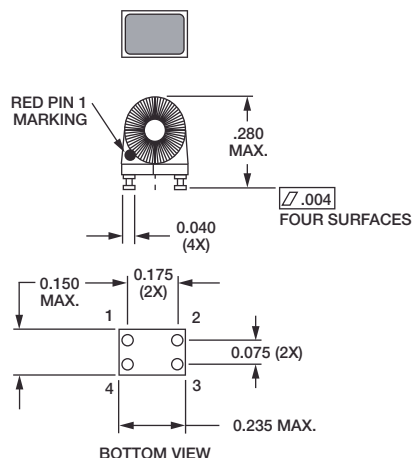
501-0912 MECHANICAL
